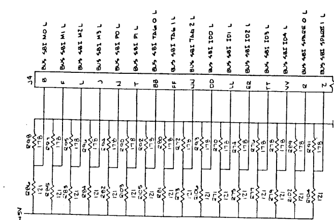
J4 TERMINATOR
